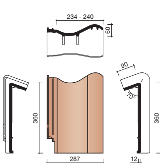
8500 CHAPERONPAN
