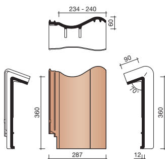
8500 CHAPERONPAN
